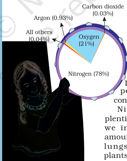
Fig. 4.1: Constituents of Air
